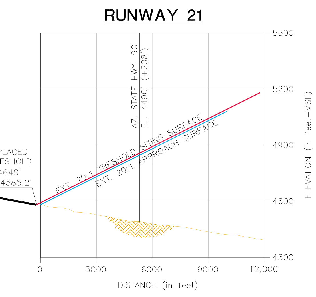
RUNWAY 3-21 APPROACH ZONES PROFILES
