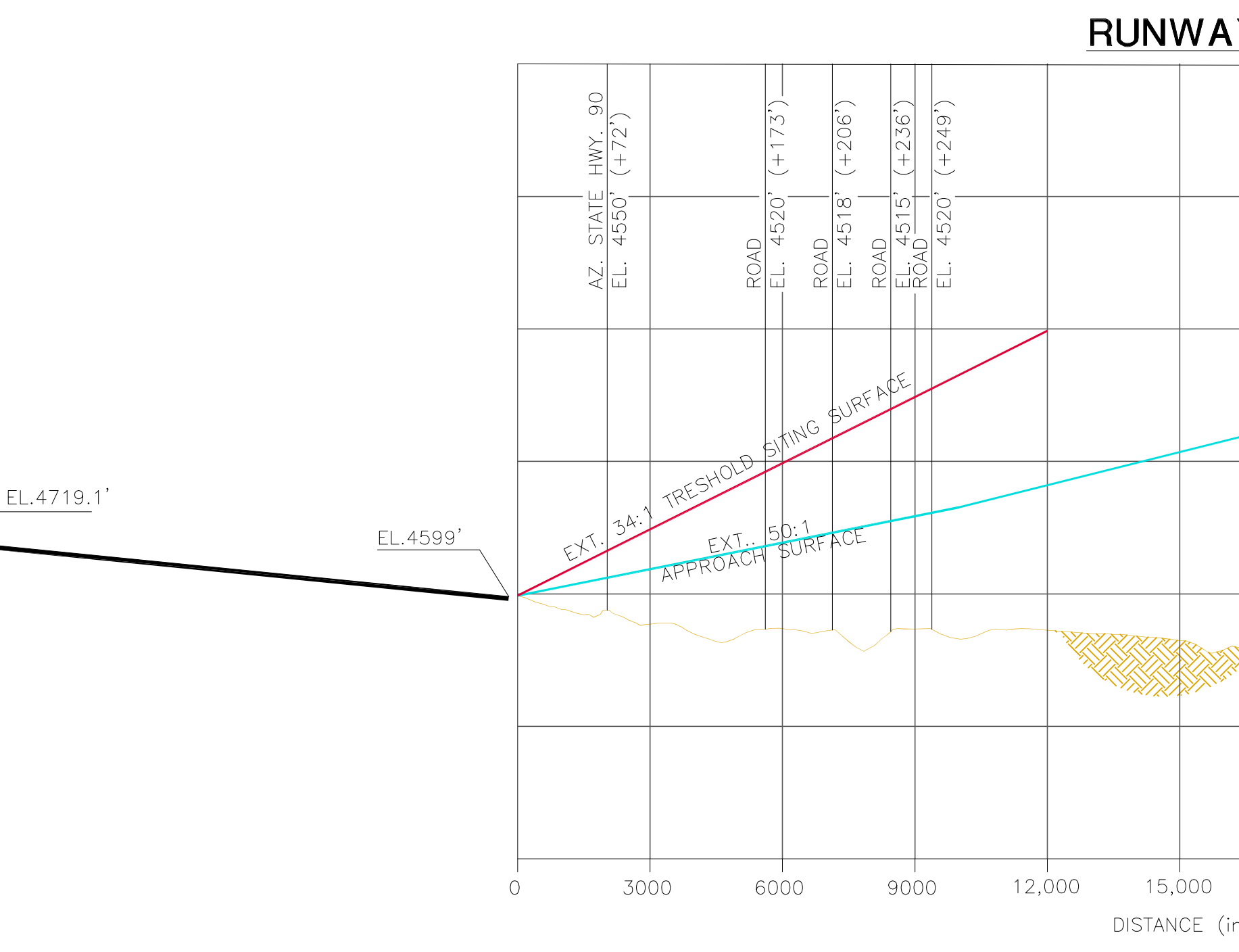
RUNWAY 8-26 APPROACH ZONES PROFILES
