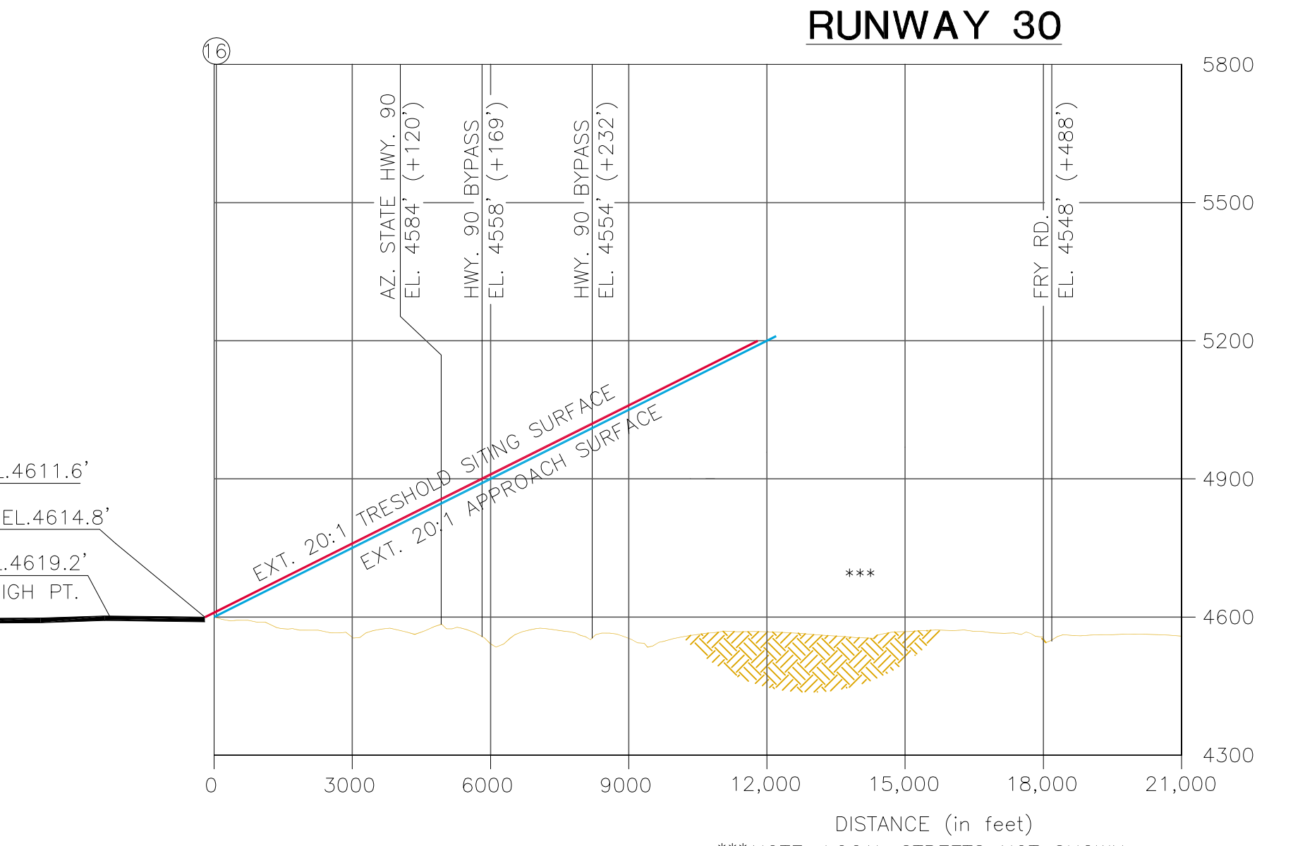
RUNWAY 12-30 APPROACH ZONES PROFILES
