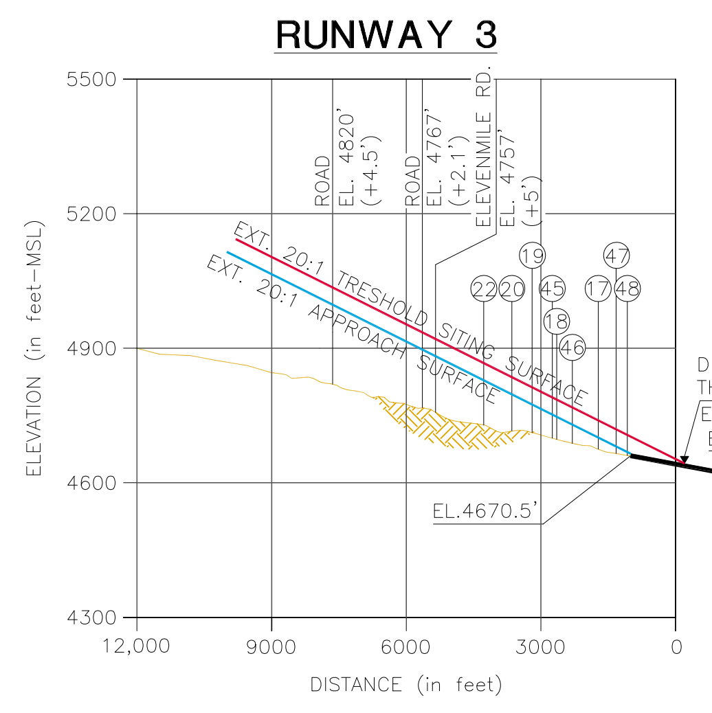
RUNWAY 3-21 APPROACH ZONES PROFILES
